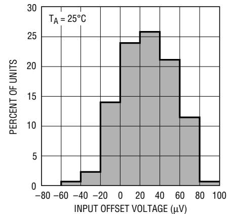
Distribution of Offset Voltage at V_S = \pm 1.0V (In All Packages)
